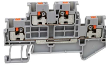
Terminal block with 4 connections UJ6-1.5/2-2
