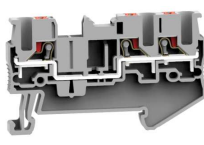
Terminal block with 3 connections UJ6-2.5/1 × 2
